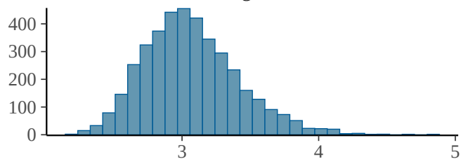
sigma
