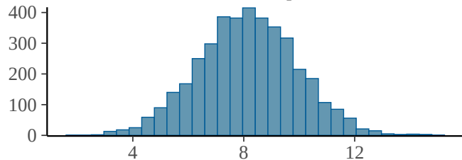
b_Intercept
