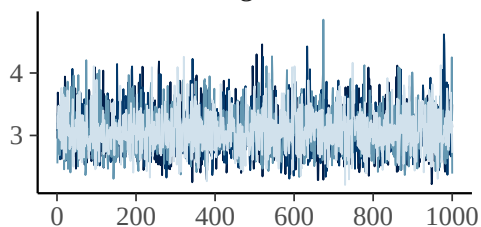
sigma
